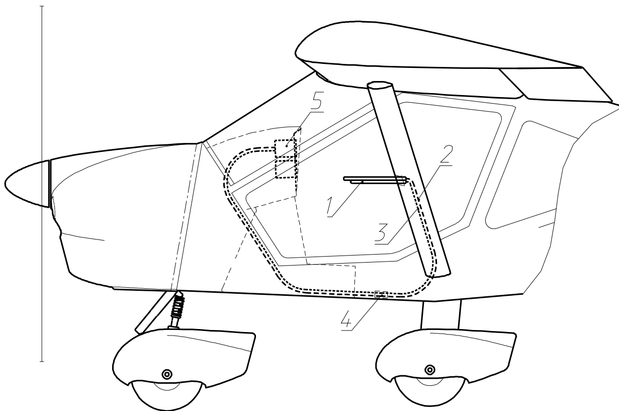
Fig. 14. Full and static pressure system
