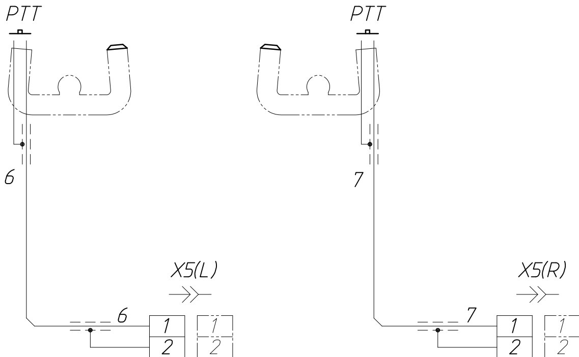
Fig. 19. Wiring diagram for installation of PTT buttons
