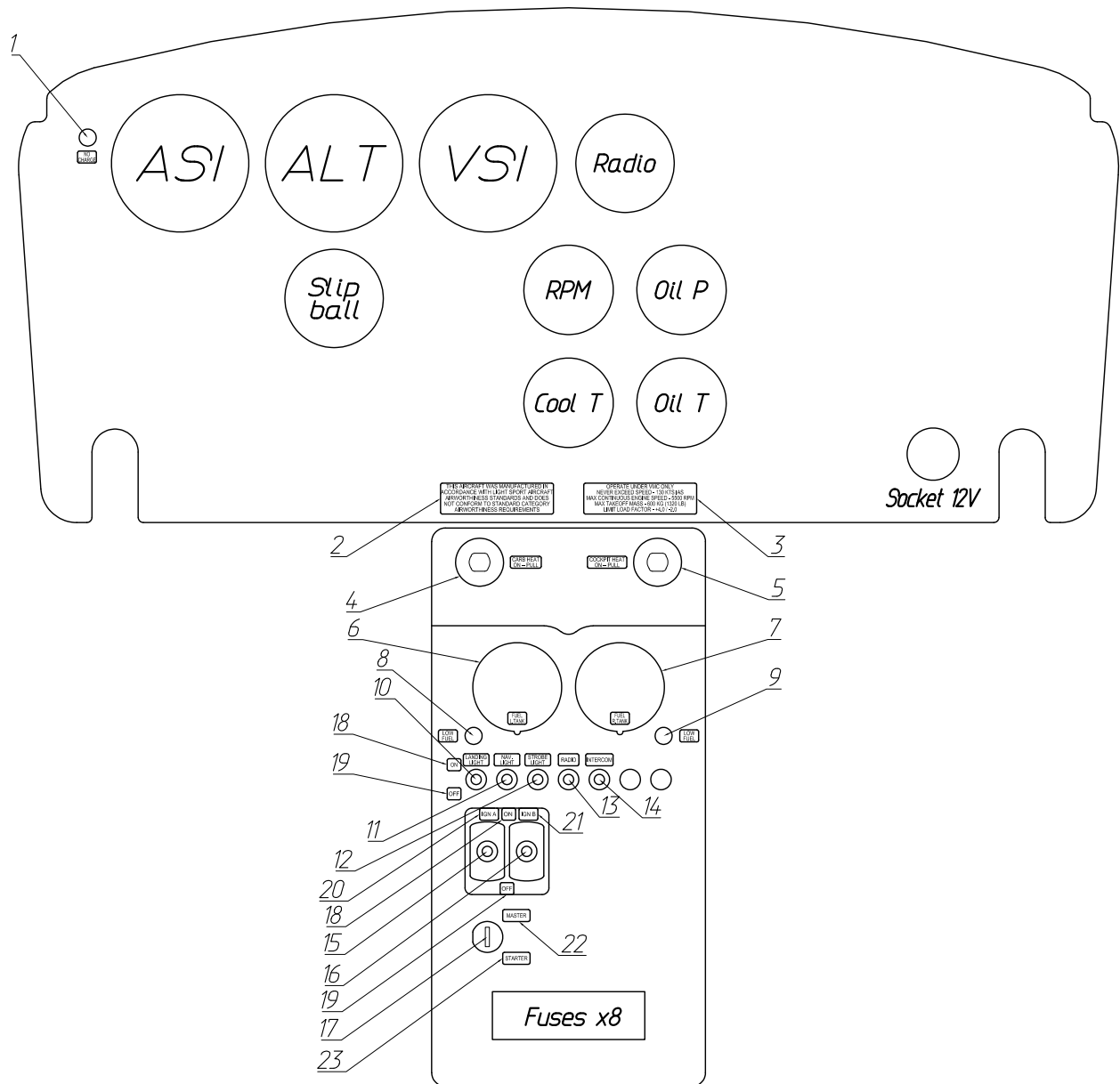
Fig. 13. Instrument panel
