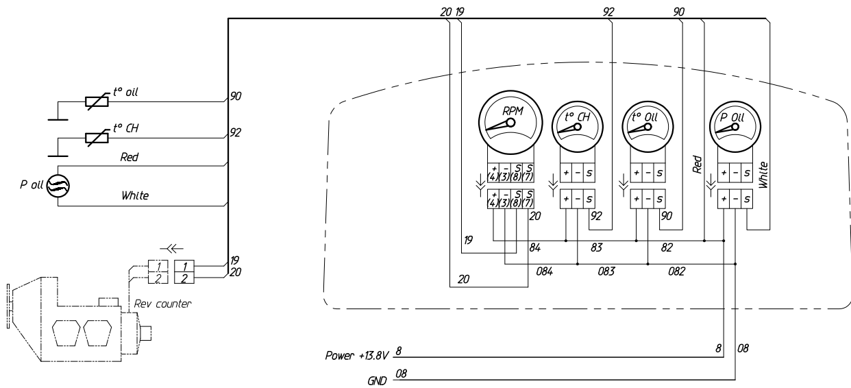
Fig. 16. Wiring diagram for installation of the analog engine instrument
