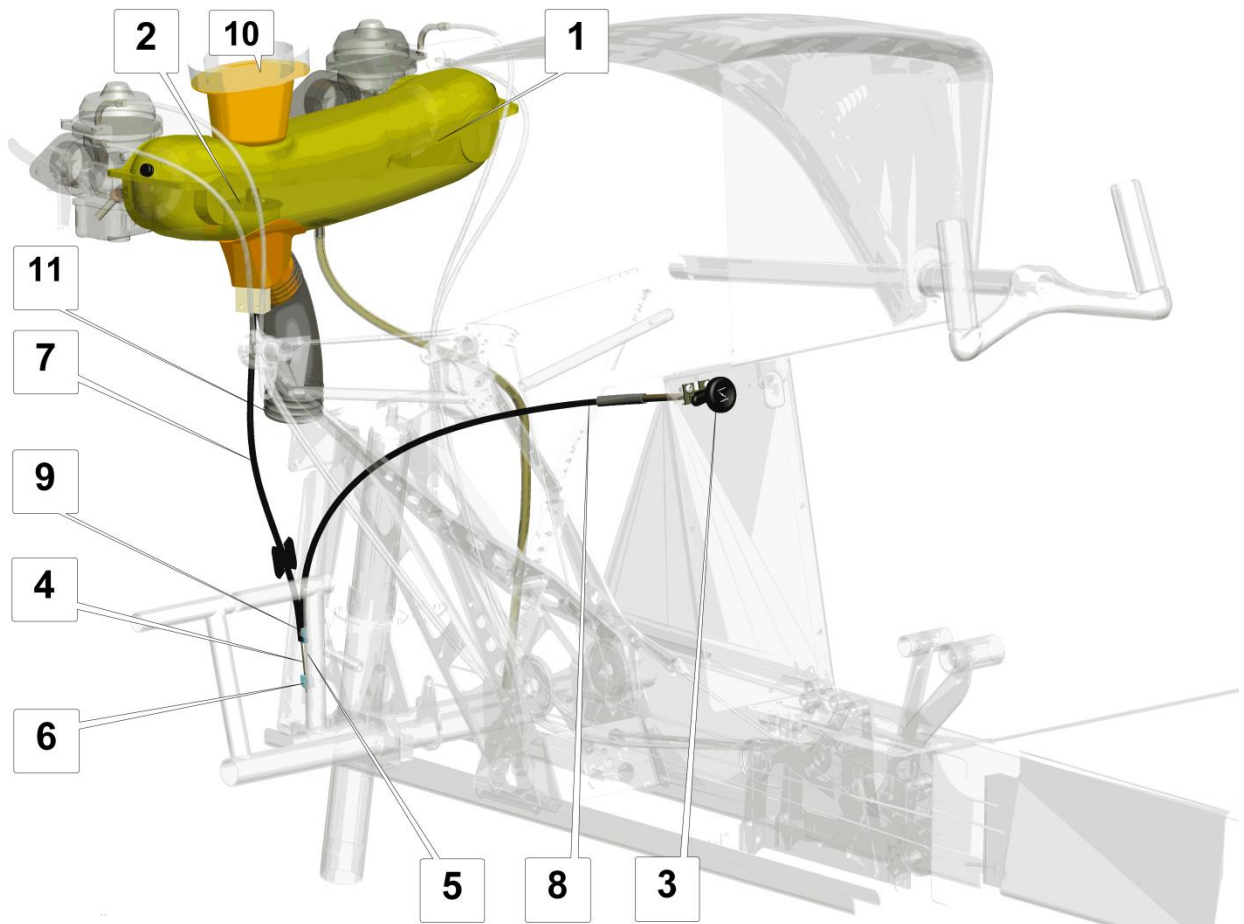
Fig. 11. Carburetor heating control
