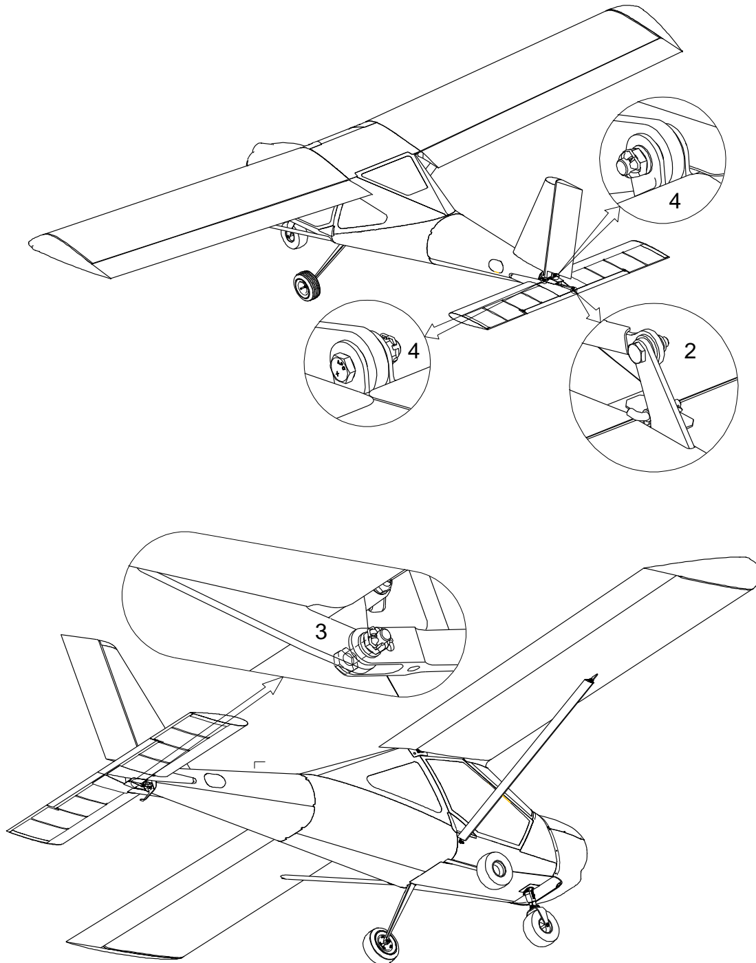
Fig. 24. Removal of the AFHT
