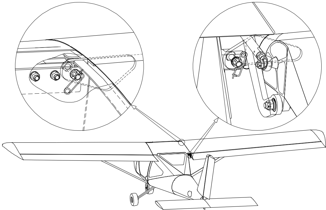
Fig. 22. Wing removal – wing-to-fuselage attachment points
