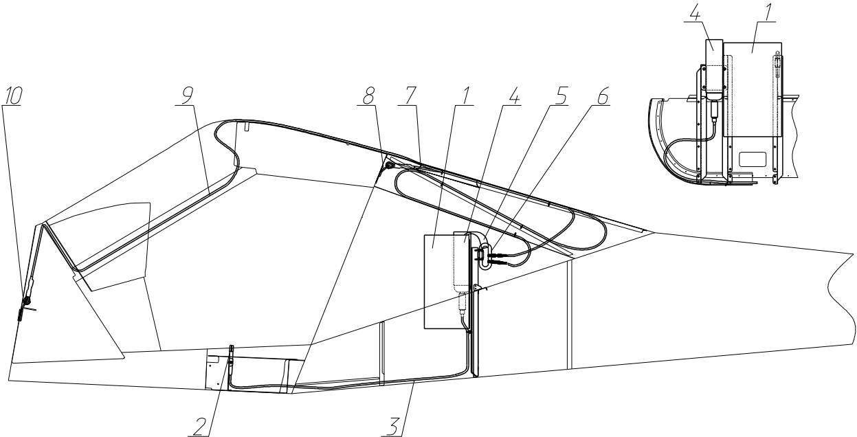
Fig. 20. Recovery system
