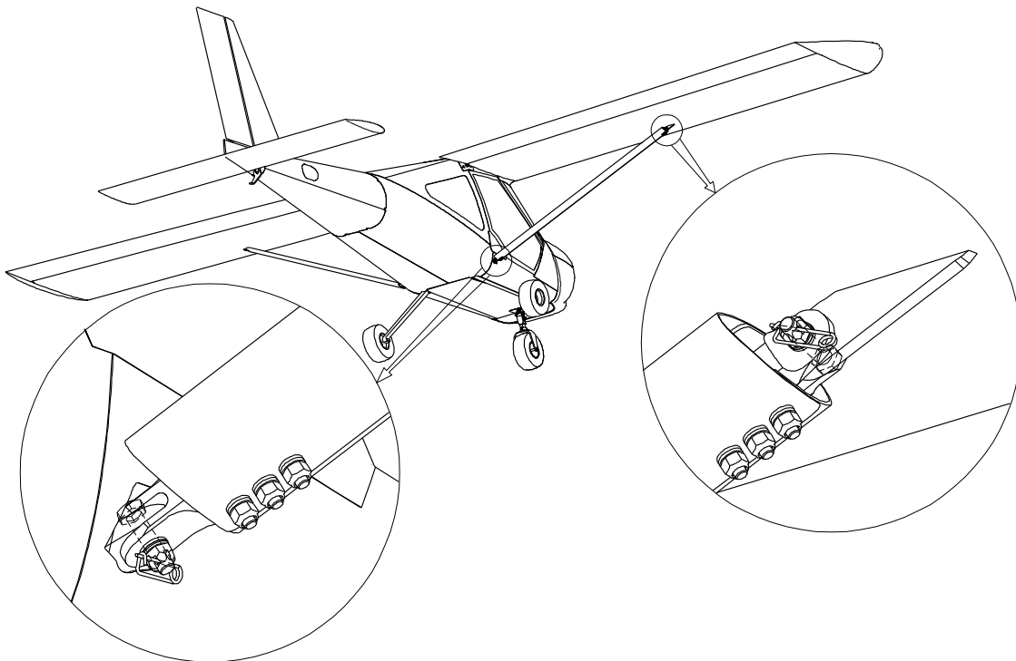
Fig. 23. Wing removal – wing strut attachment points
