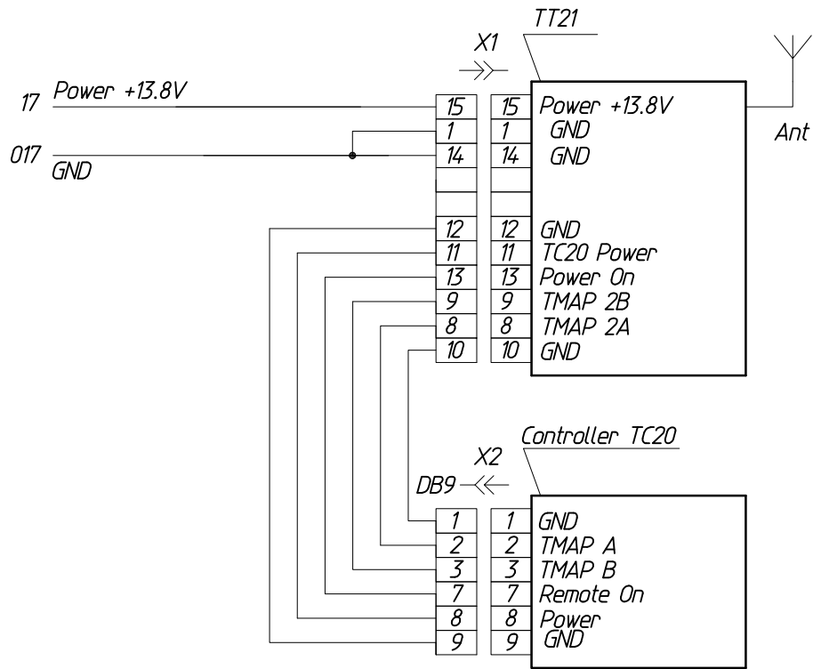
Fig. 18. Wiring diagram for installation of the Trig TT21 transponder
