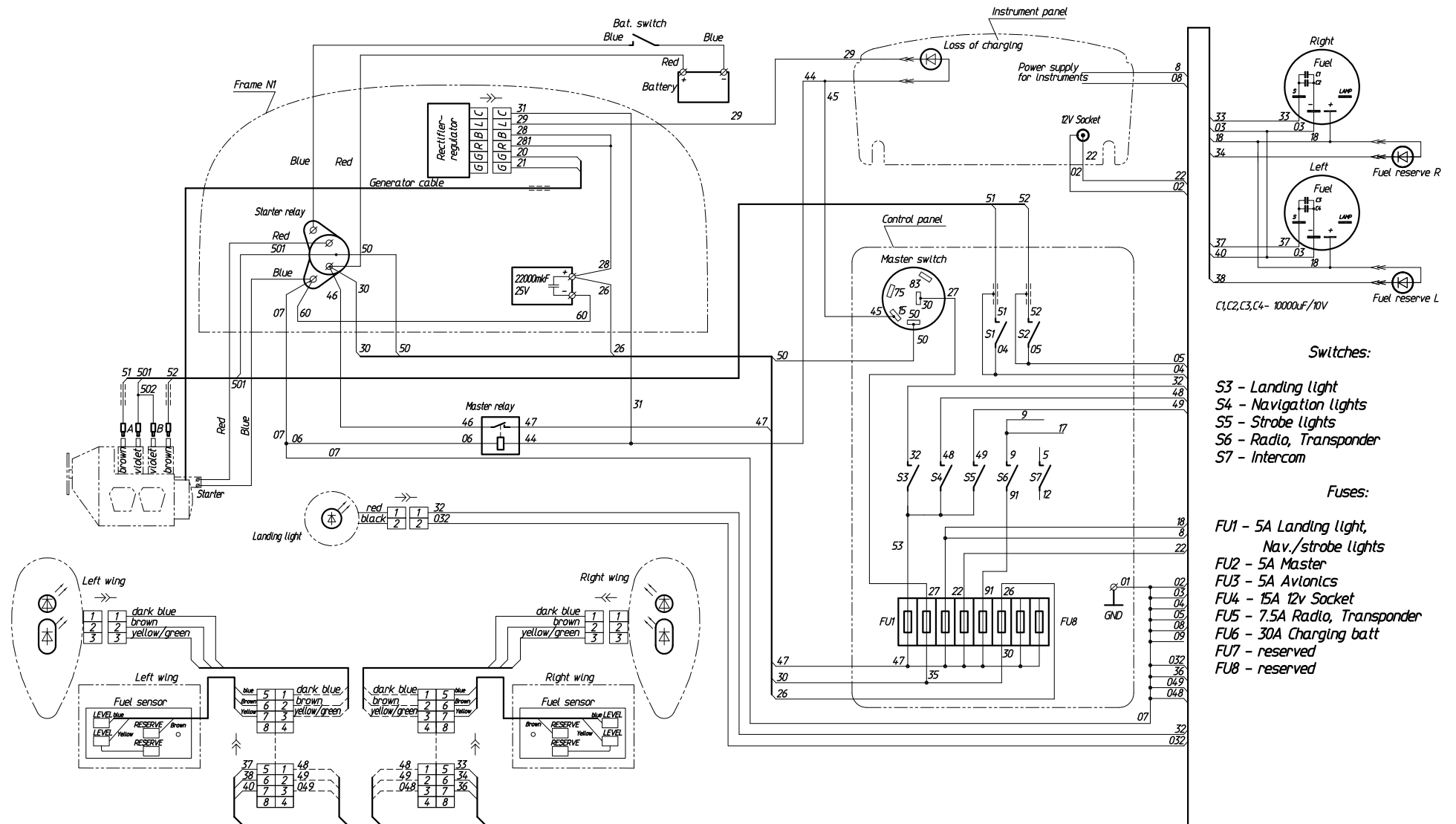
Fig. 15. Wiring diagram of A32 electrical system (main)
