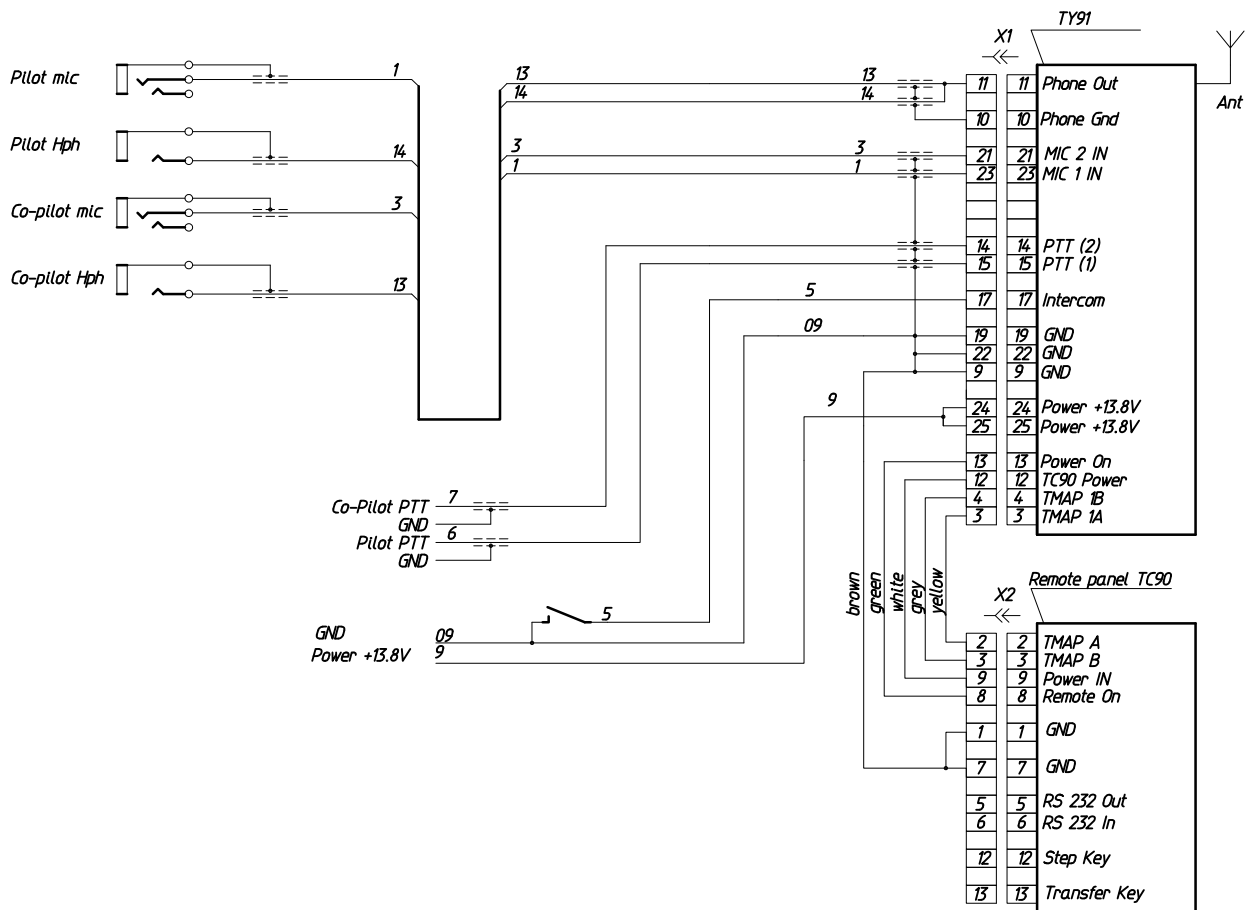
Fig. 17. Wiring diagram for installation of the Trig TY91 radio
