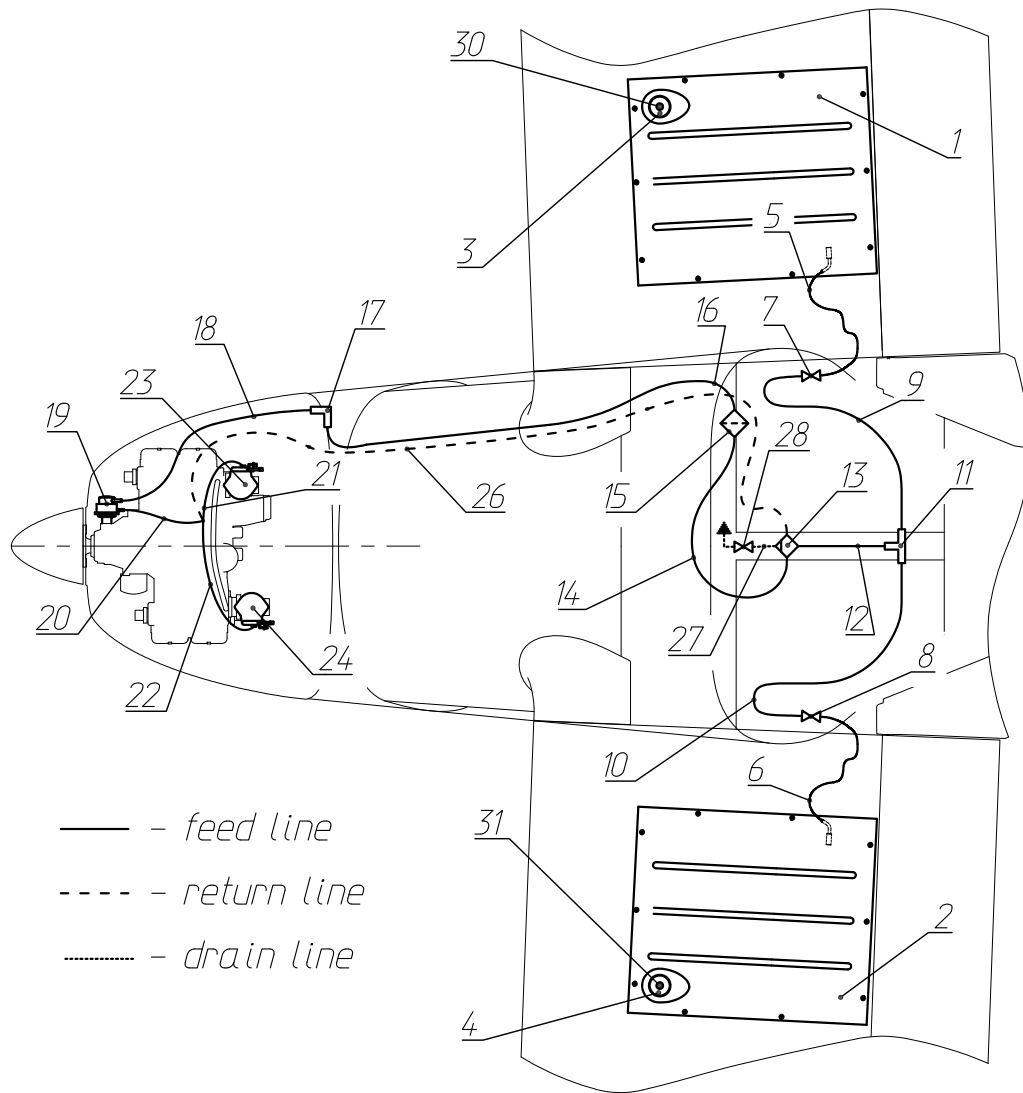
Fig. 3. Fuel system schematic
